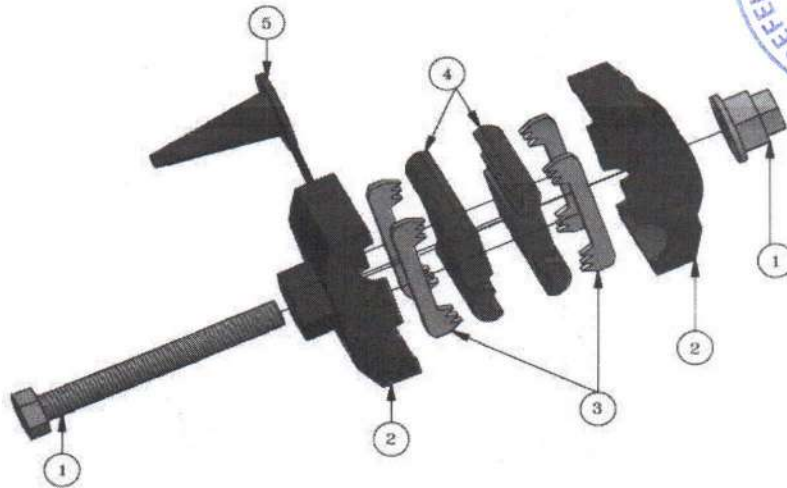
VISTA EXPLODIDA
