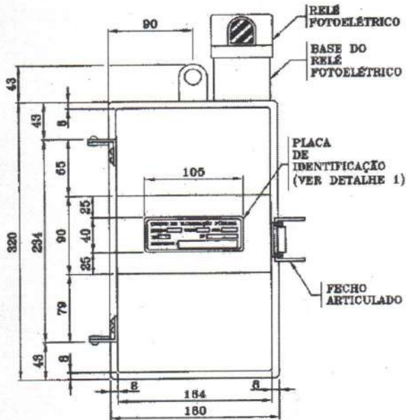
VISTA FRONTAL
